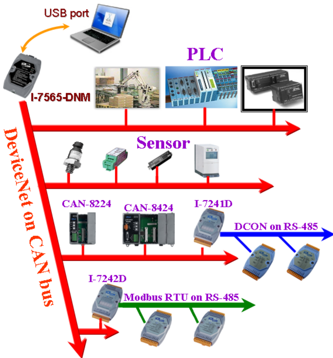
Figure 1.3 Application architecture
