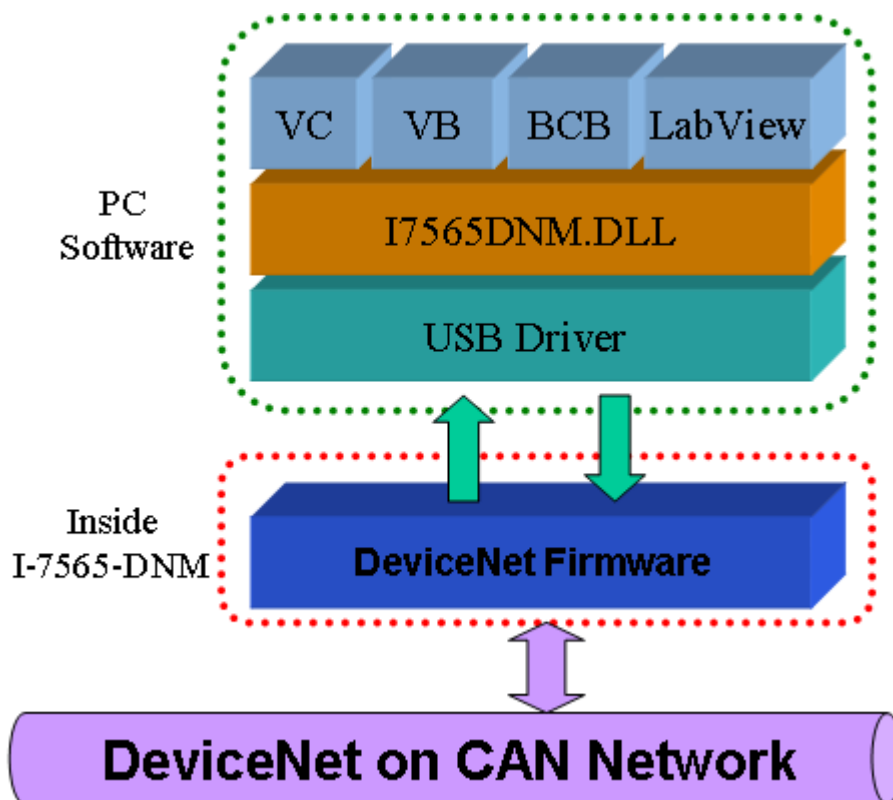
Figure 1.2 I-7565-DNM architecture.
