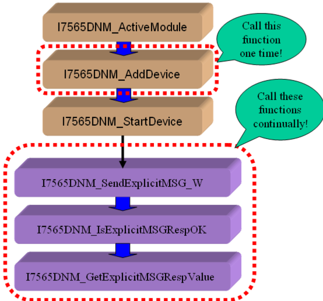
Figure 3.9 “SendExplicitMSG_W” Diagram
