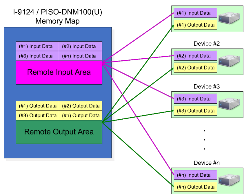
Figure 3.10 The Memory Mapping of the I-9124
