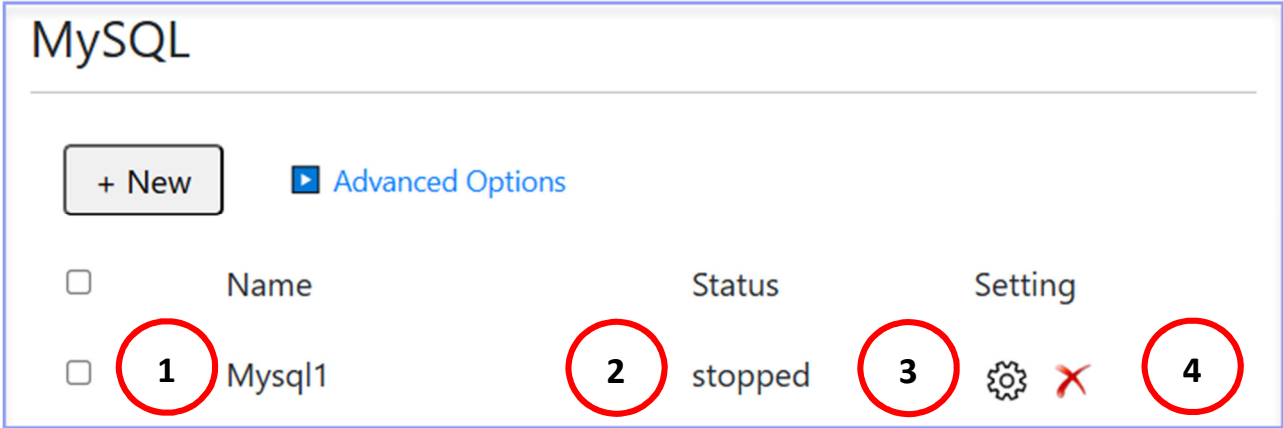
Figure 4-24 MySQL Setting
