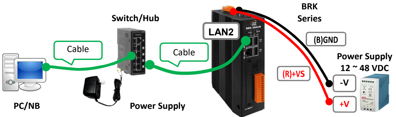
Figure 2-1 Hardware Wiring
