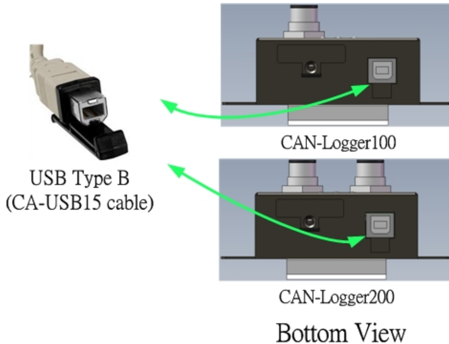
Figure 4-1 Wire connection of the USB
