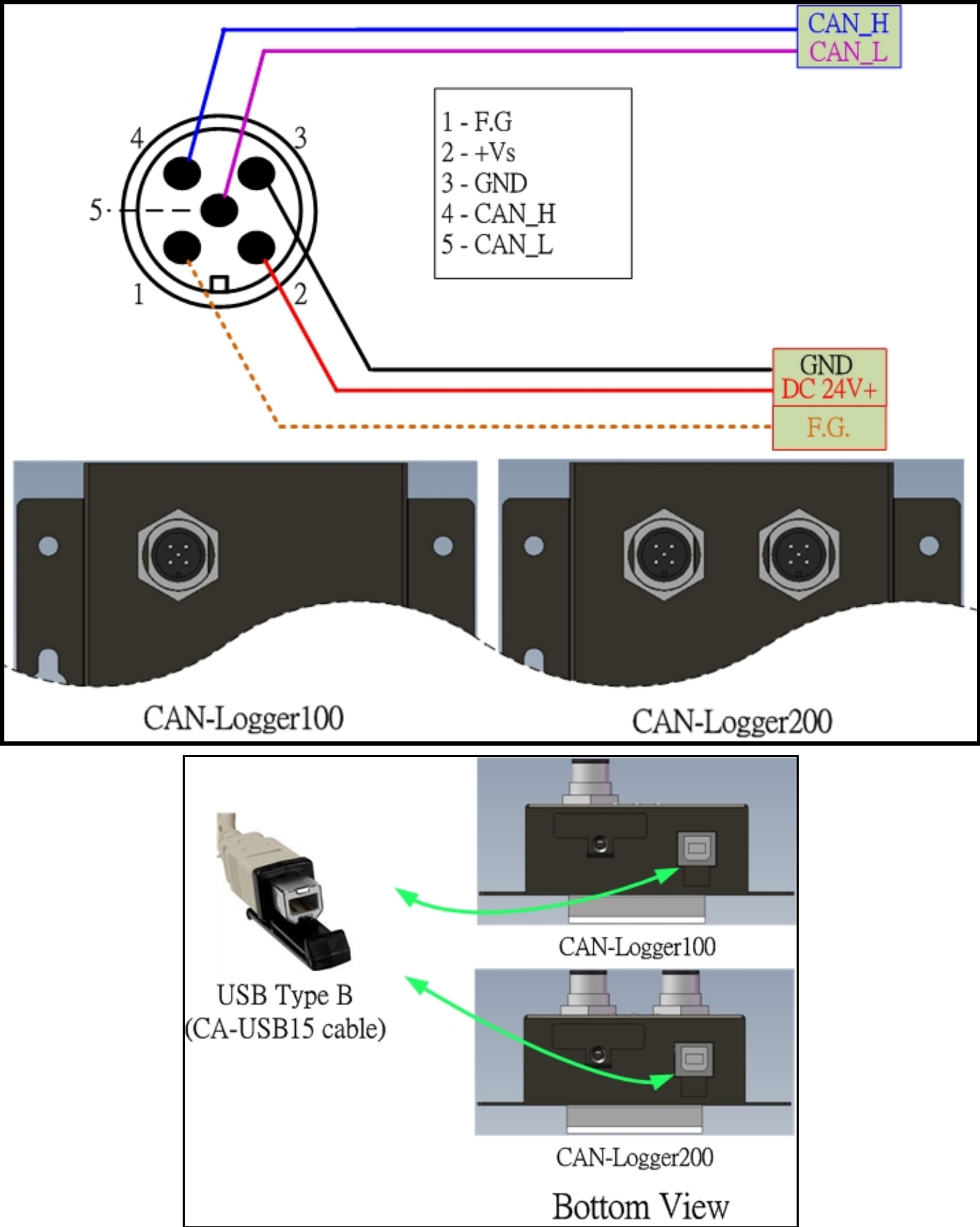
Figure 2-42 Wire Connection for CAN-Logger series
