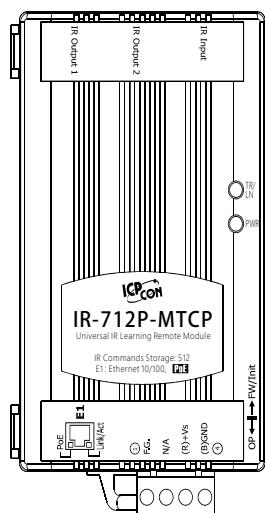
IR Interface of the IR-712-MTCP
