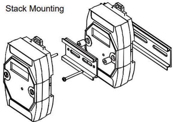
Din-Rail Mounting
