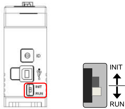
Figure 2-6 The hardware setting for enabling firmware update functionality
