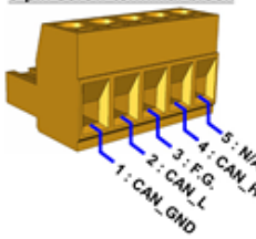
5-pin screw terminal block
