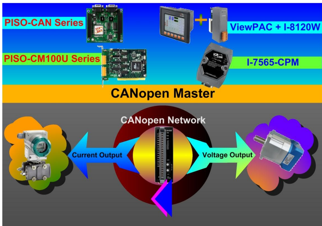
Figure 1-2 Application Structure
