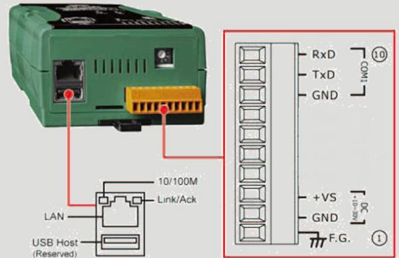
Pin Assignment
