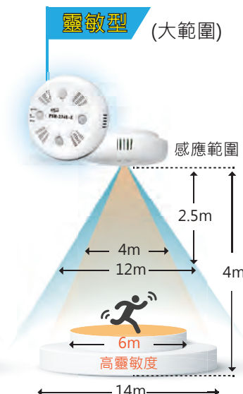
PIR-234L PIR-234L-WF
