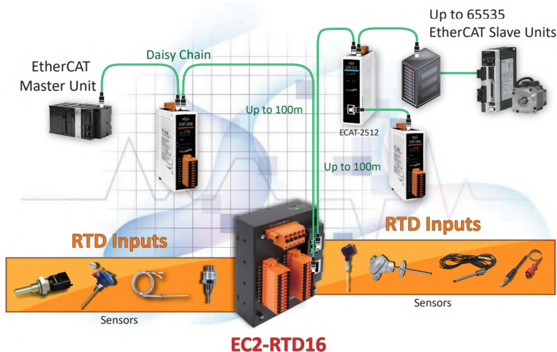
Figure 1.1 Typical Application of EC2-AI Module
