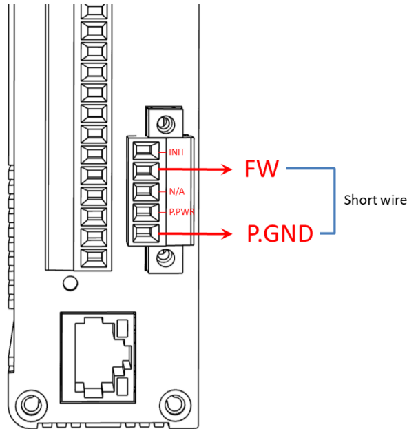
Figure 11 BNET-2119M FW & P.GND Pin
