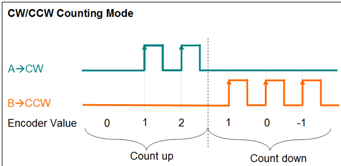
圖 28: Clockwise/ Counterclockwise counting mode
