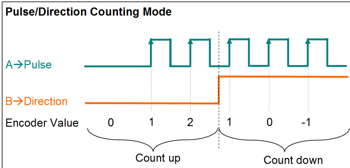
圖 27: Pulse/Direction counting mode
