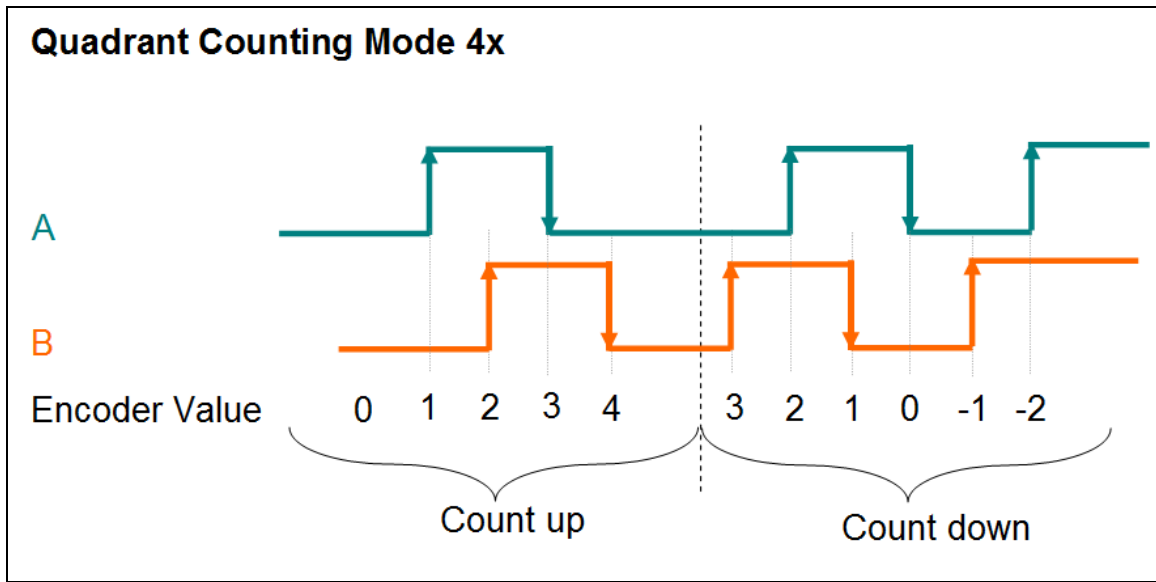
圖 29: Quadrant counting mode
