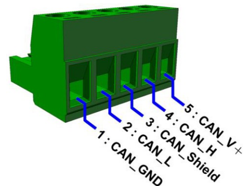
5-pin screw terminal block
