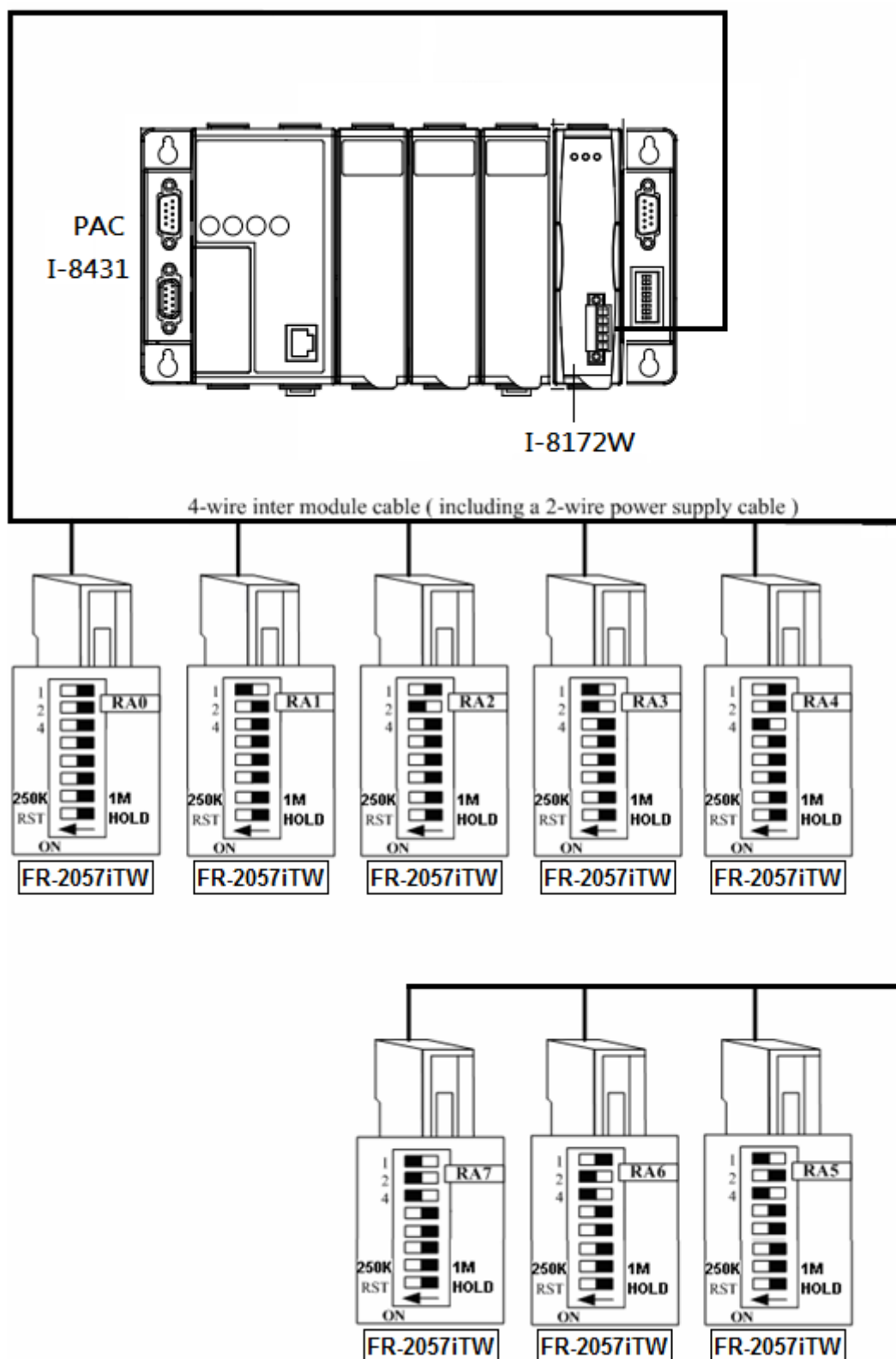
Figure 2.7 FRnet communication controller and distributed IO modules
