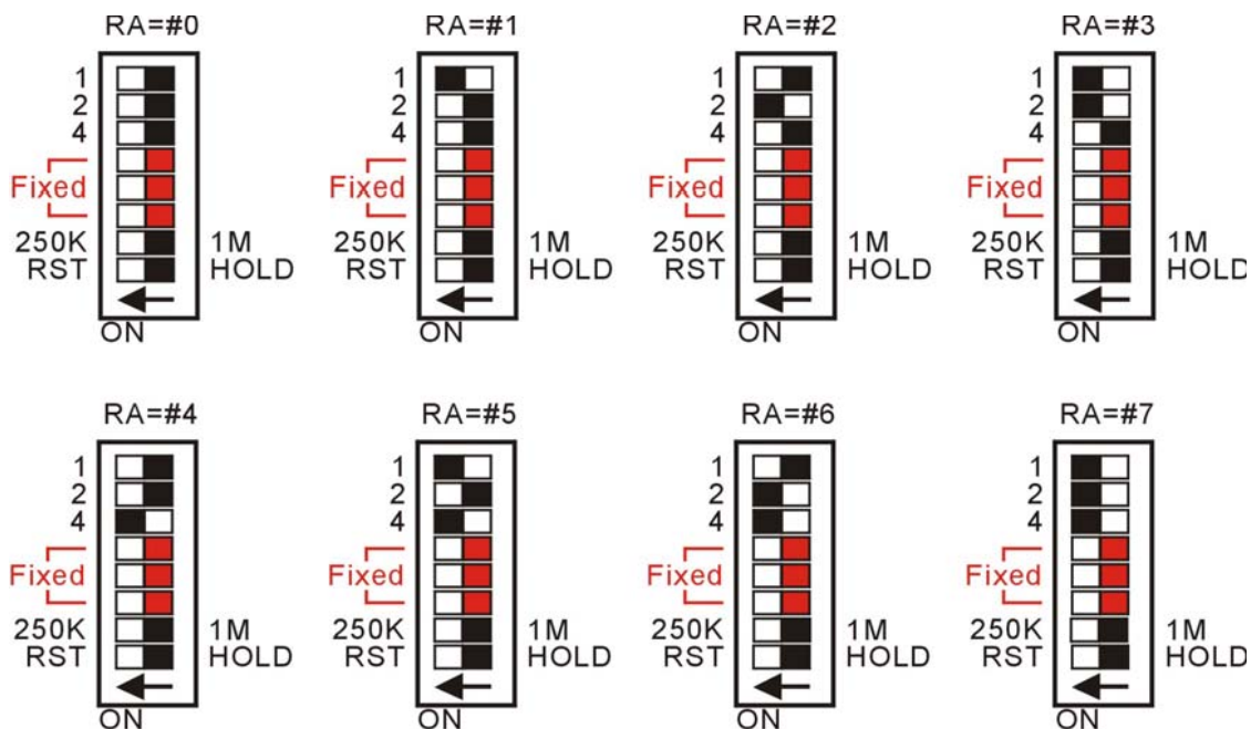
Figure 2.5 Receiver address setting.
