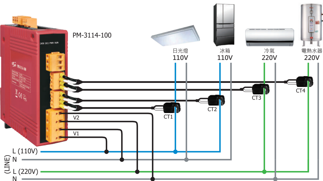
CT1 and CT2 for reference voltage V1; CT3 ~ CT4 for reference voltage V2.
