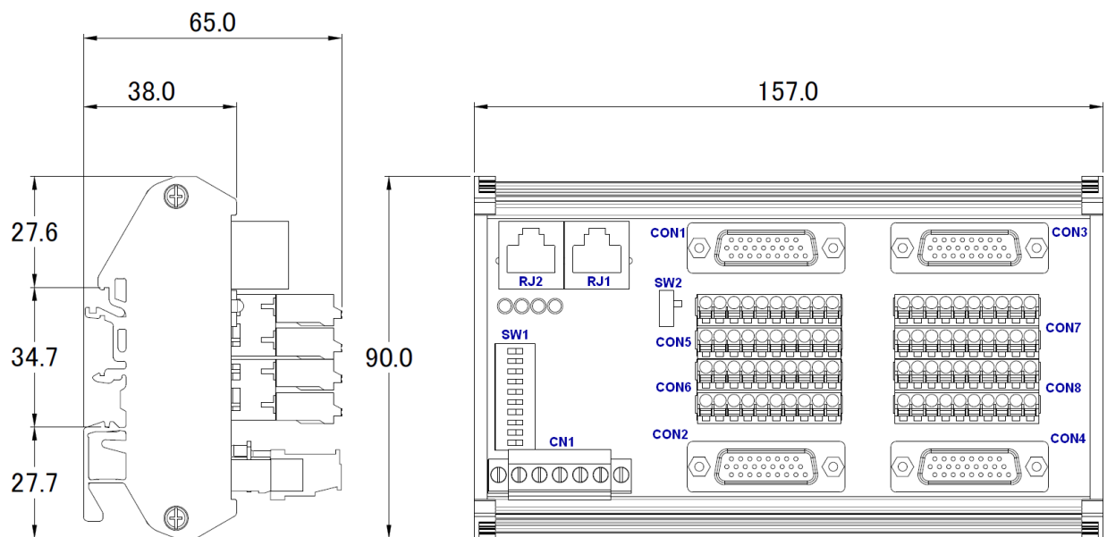
Dimension of MN-MP4U-DIN
