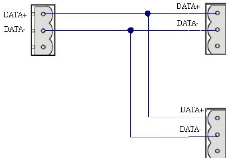
❖ RS-485 connection
