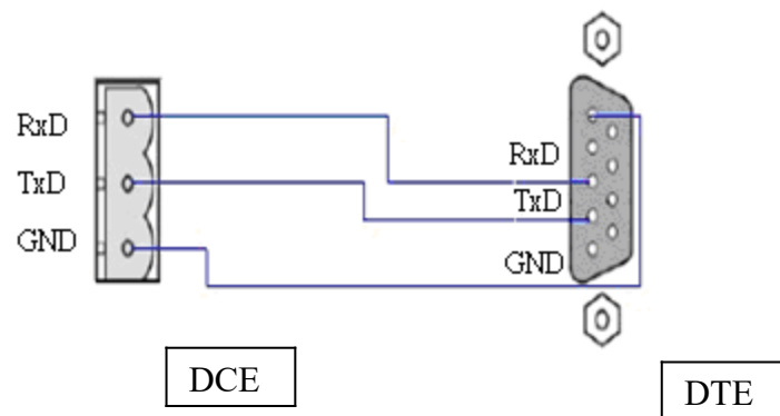
❖ RS-232 Three-wire connection
