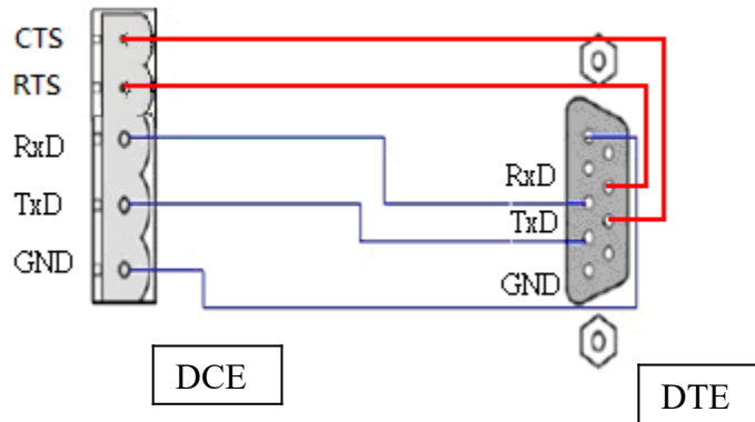
❖ RS-232 Five-wire connection
