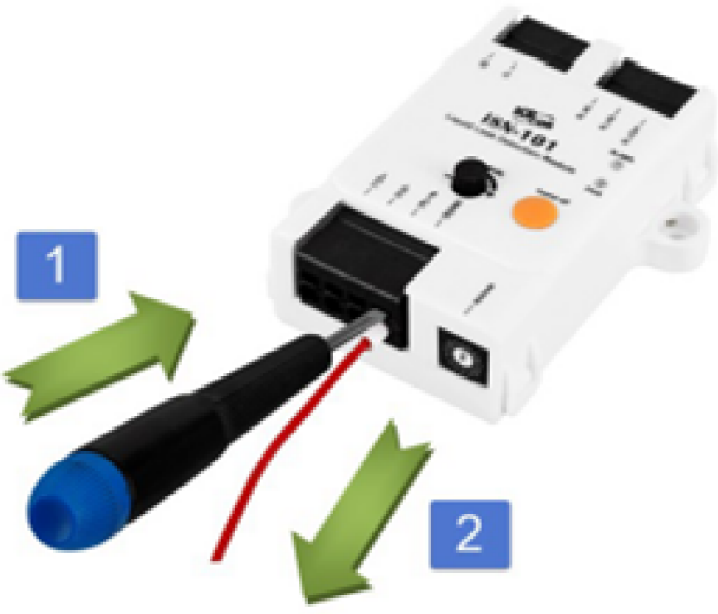
Remove the wire
