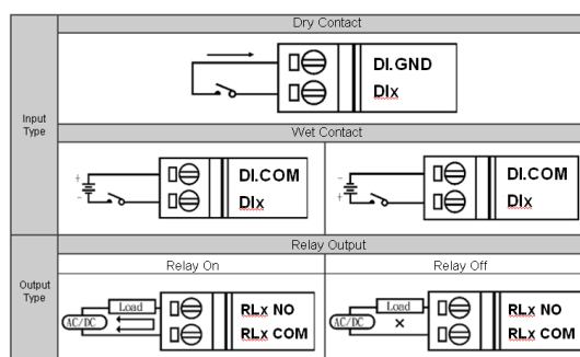
Wire Connection
