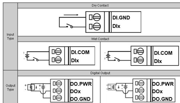
Wire Connection
