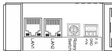
Wire Connection
