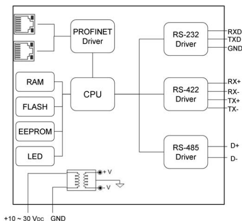
I-7580 Internal I/O Structure
