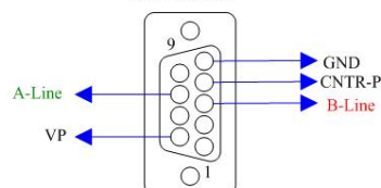
Female D-Sub Connector
