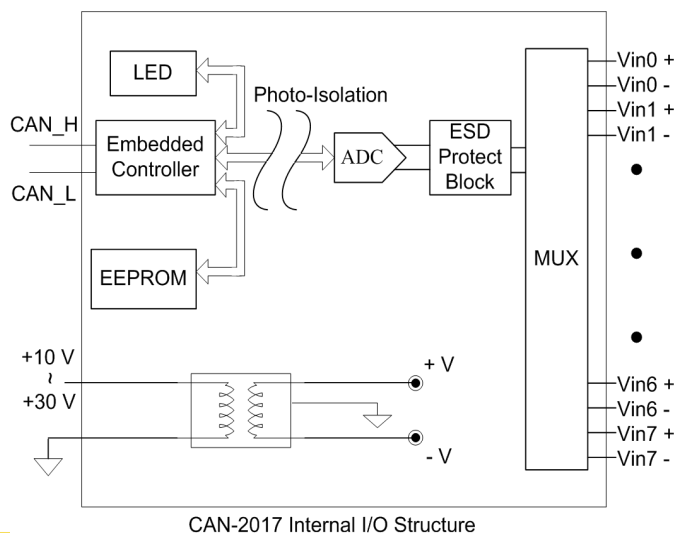
CAN-2017 Internal I/O Structure
