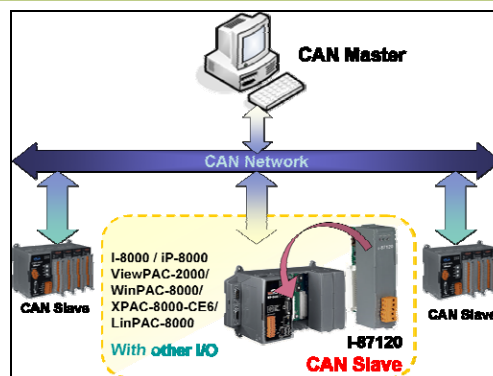
I-87120 is as CAN slave
