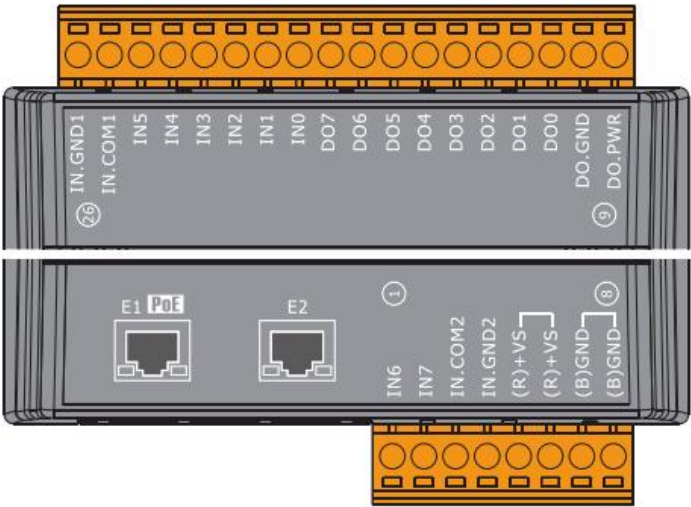
ET-7255/PET-7255
