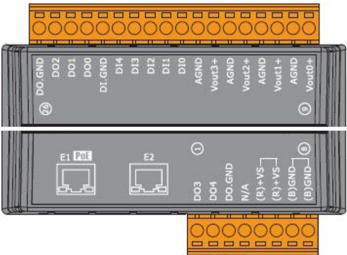
ET-7224/PET-7224
