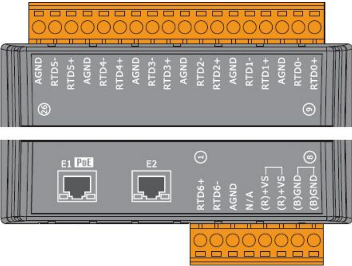
ET-7215/PET-7215
