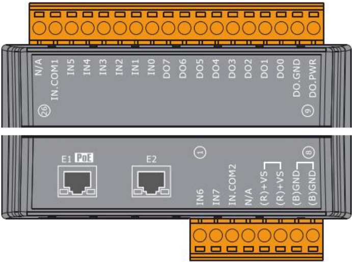
ET-7252/PET-7252
