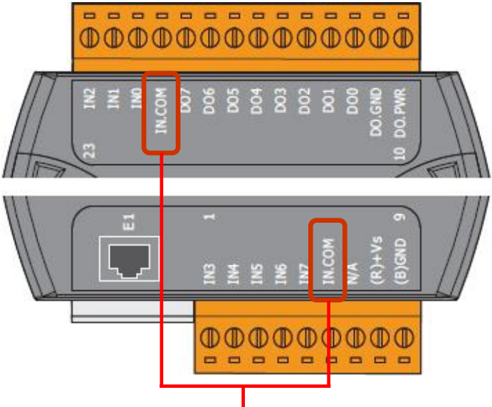
ET-7052/PET-7052
