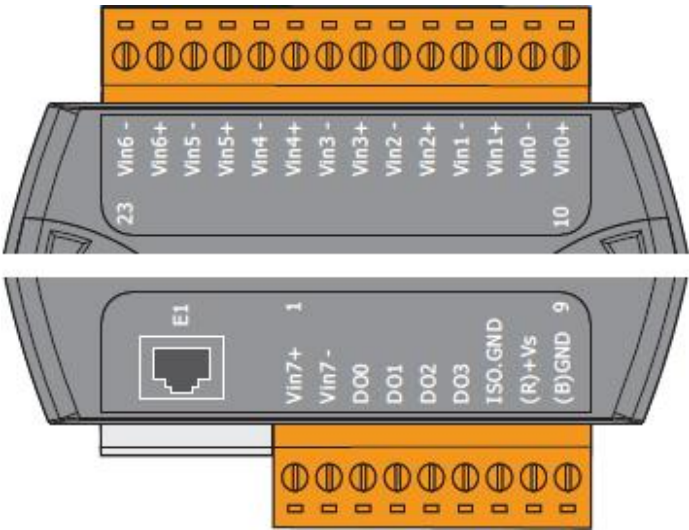
ET-7217/PET-7217
