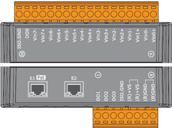
ET-7217/PET-7217
