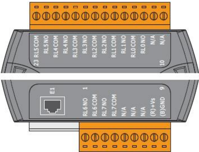
ET-7267/PET-7267
