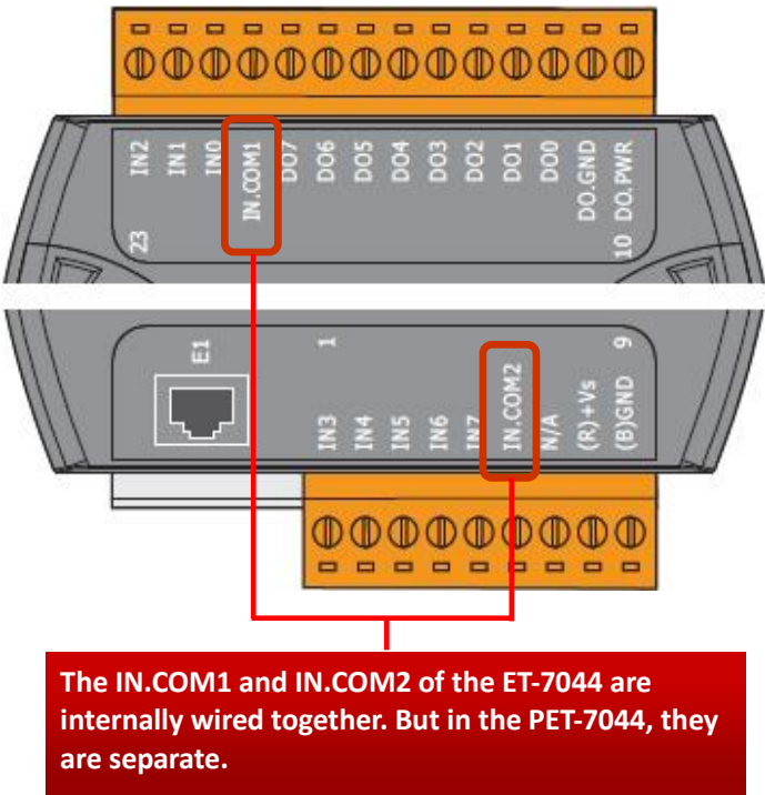
ET-7044/PET-7044
