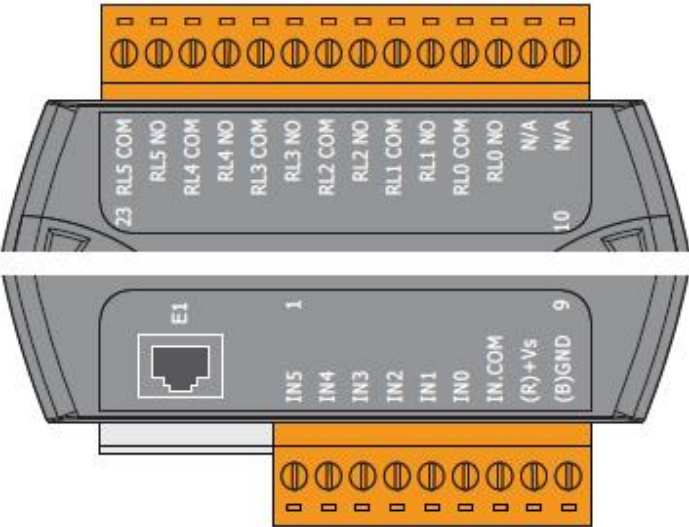
ET-7260/PET-7260
