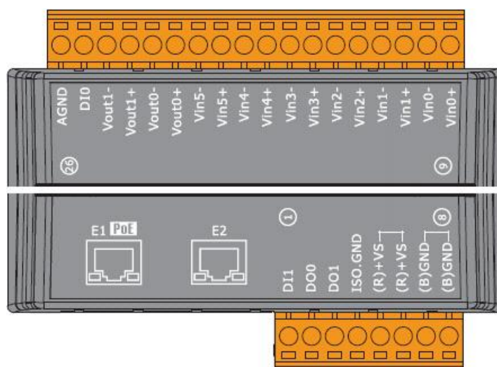
ET-7226/PET-7226
