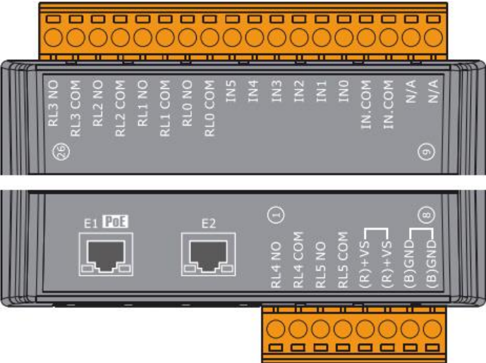
ET-7260/PET-7260
