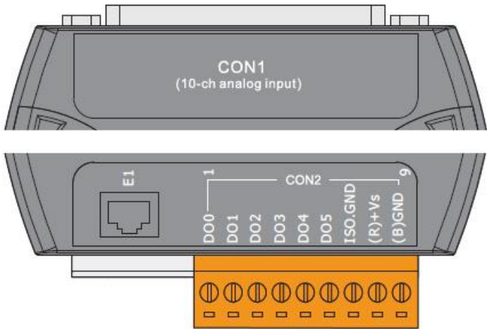
ET-7019Z/PET-7019Z
