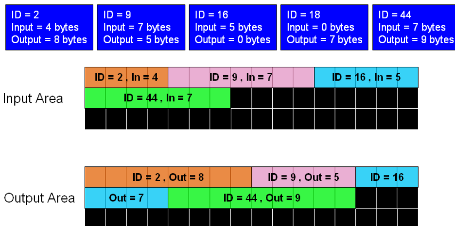
Figure 3.12 The example of the I-8124W memory mapping
