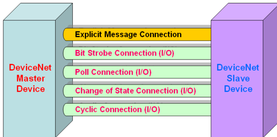
Figure 1.4 DeviceNet Messaging
