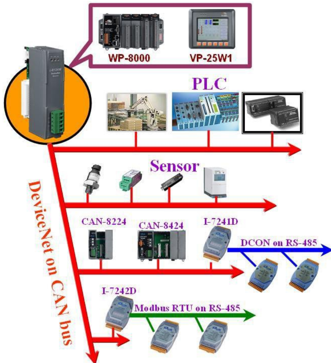
Figure 1.3 Application architecture
