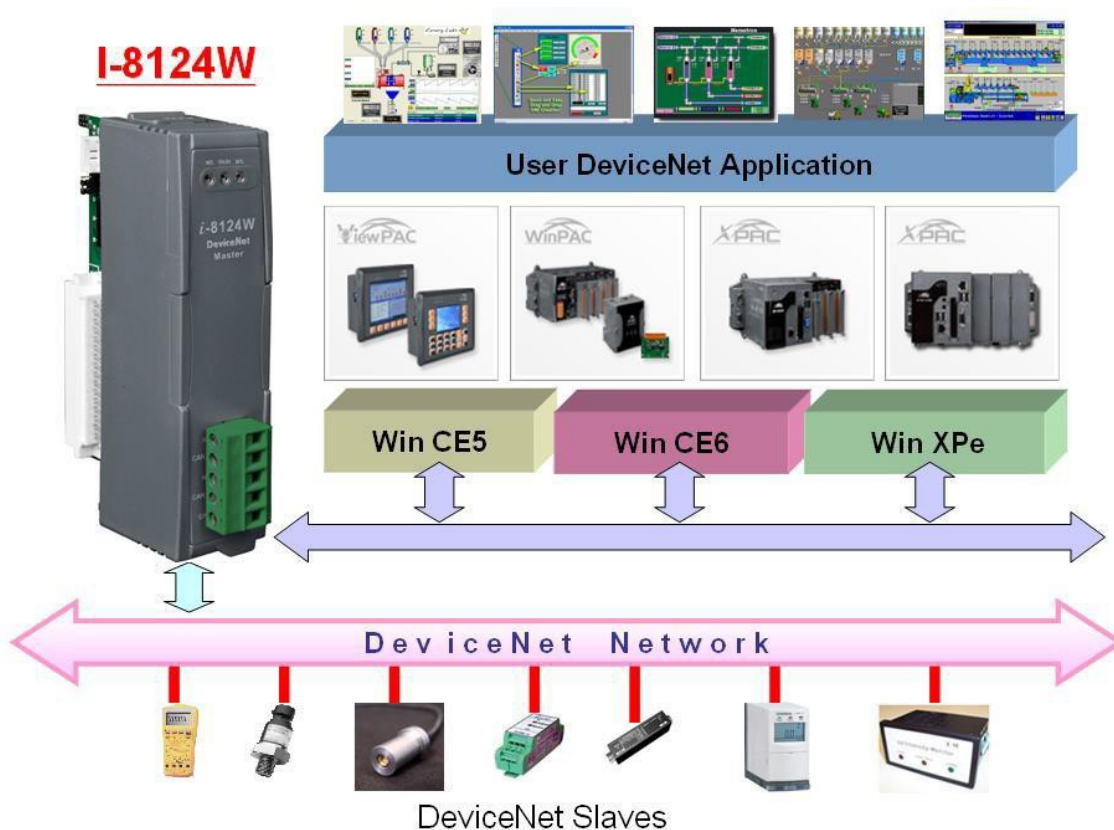
Figure 1.2 I-8124W architecture
