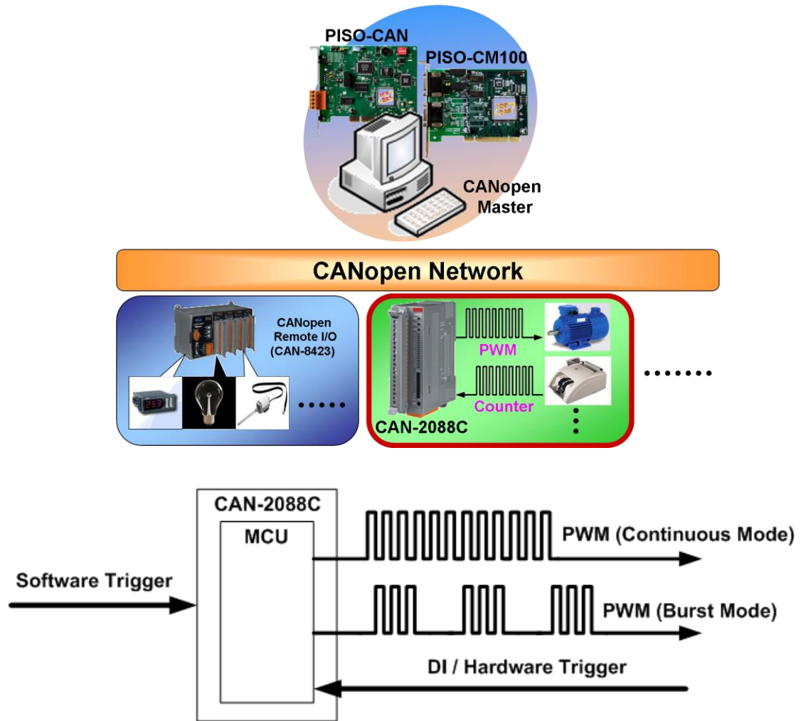
Figure 1-2 Application Structure
