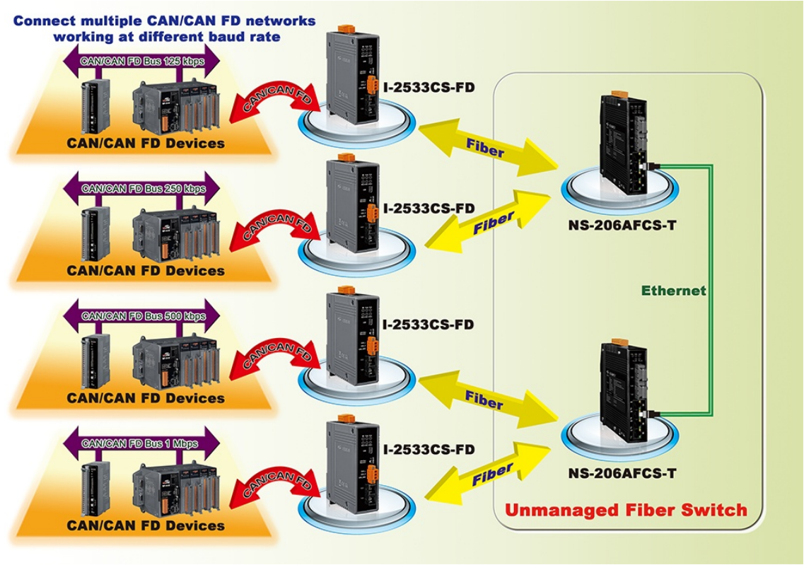
RAW Data to CAN/CAN FD communication
