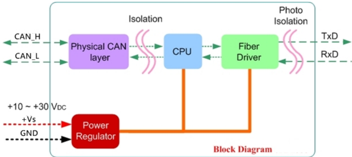
Figure 2-1-1 Block Diagram of I-2533T-FD-UL series
