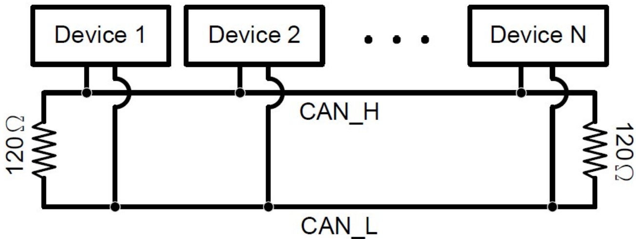
Figure 2.6-1 CAN bus network topology
