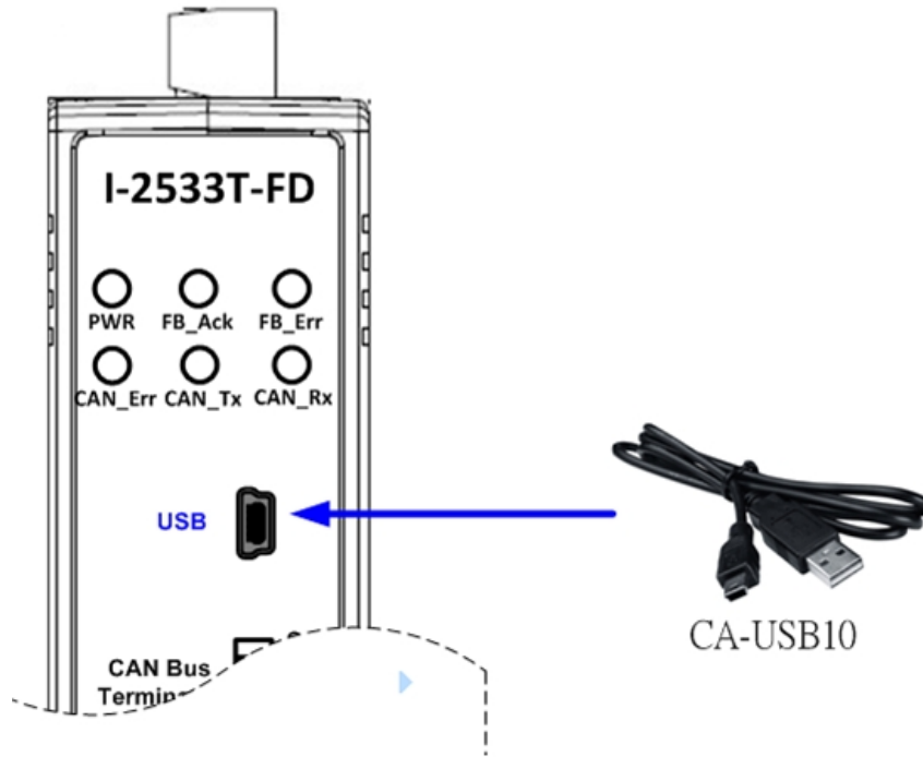
Figure 4-2-1 Wire connection of the USB
