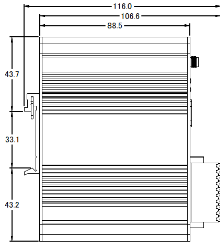
Left view
