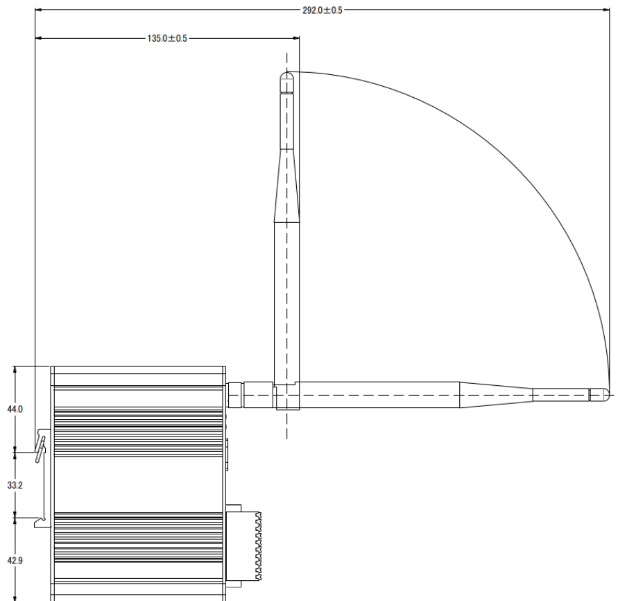
Antenna installation diagram (90 degrees and 0 degrees)
