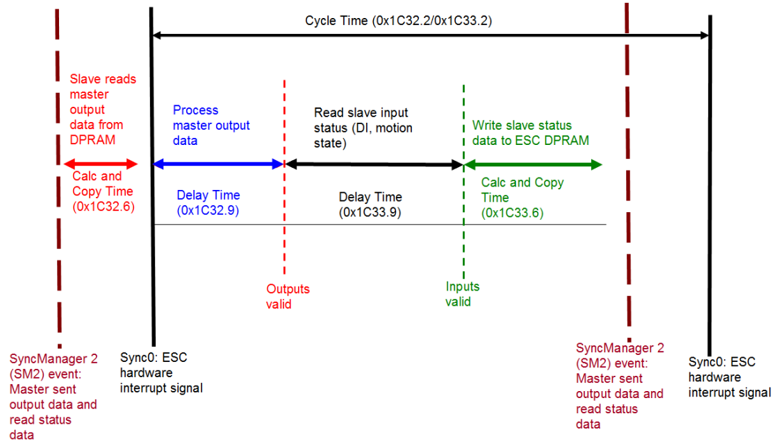
Figure 11: Internal slave processing sequence in DC mode
