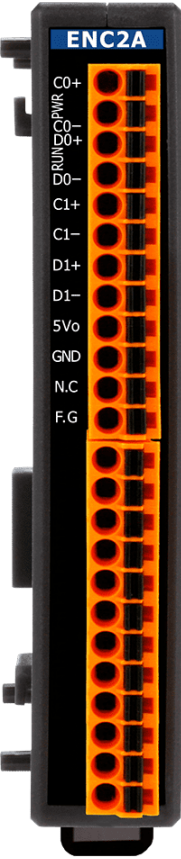
Figure 4: EC4-ENC2A side view with encoder inputs
