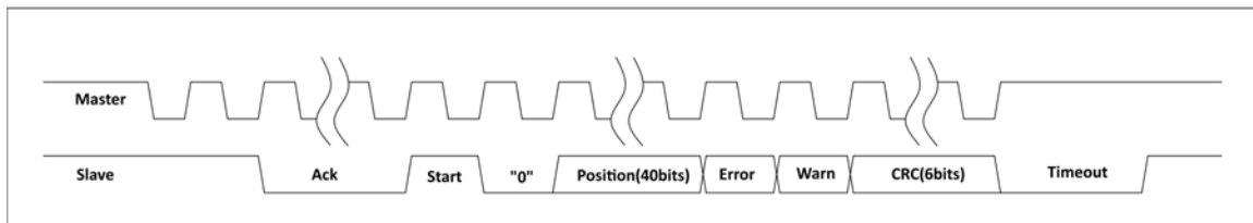
Figure 19: BiSS-C mode (unidirectional)
