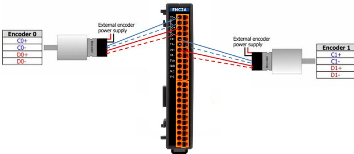
Figure 5: EC4-ENC2A encoder connection
