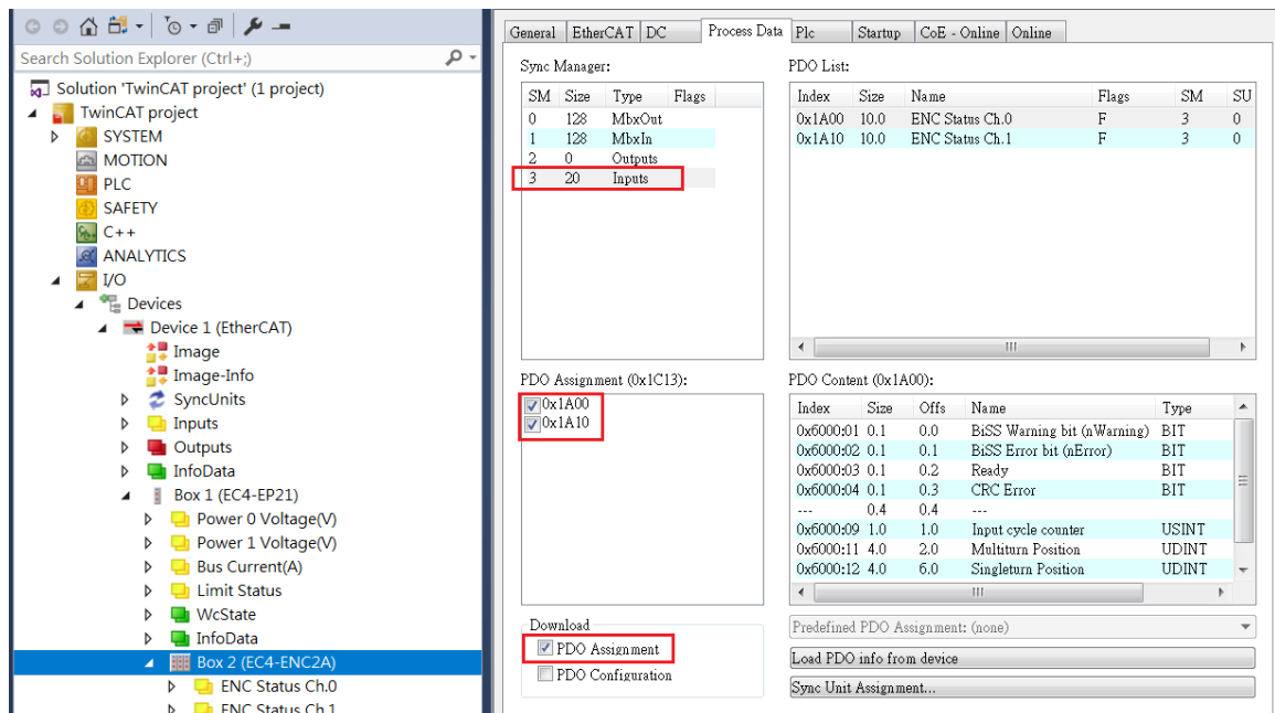
Figure 16: Predefined PDO assignment selection
