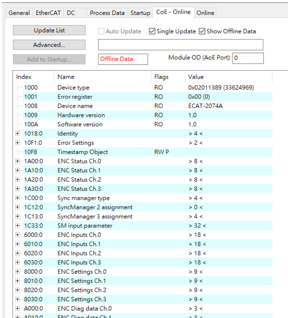
Figure 23: "CoE - Online " tab
