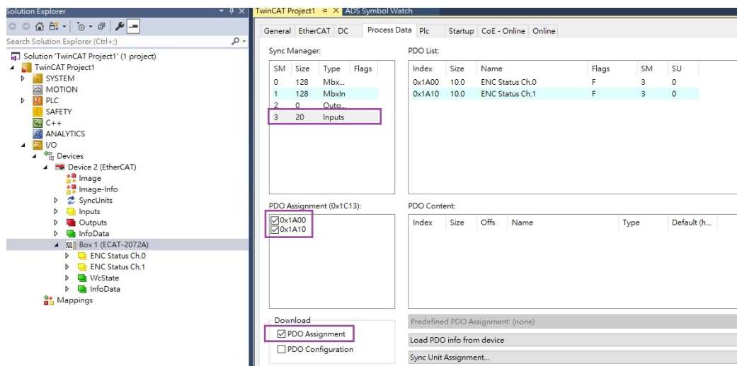
Figure 19: Predefined PDO assignment selection
