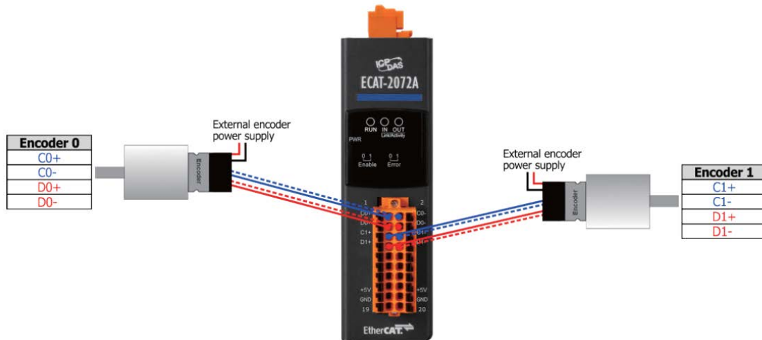
Figure 7: ECAT-2072A encoder connection
