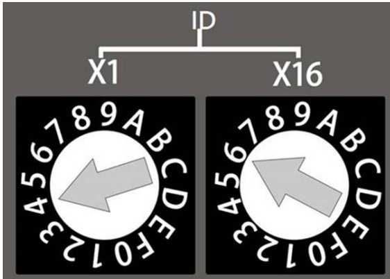
Figure 4: ECAT-2072A alias rotary switch
