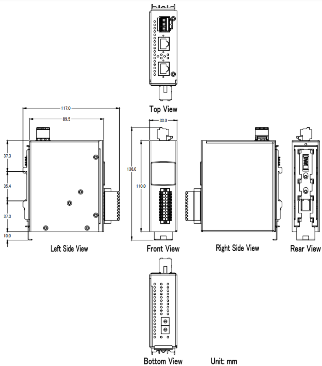
Figure 1: Dimensions of the ECAT-2072A
