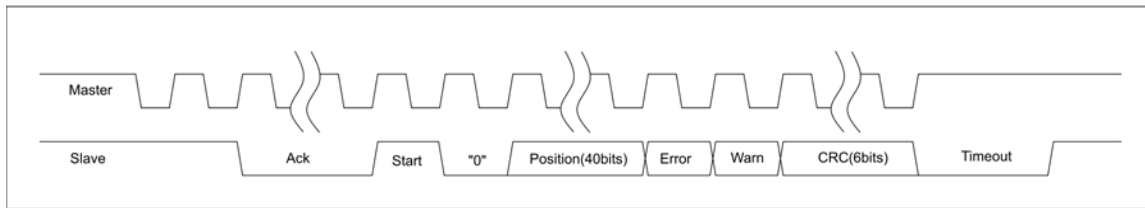
Figure 22: BiSS-C mode (unidirectional)
