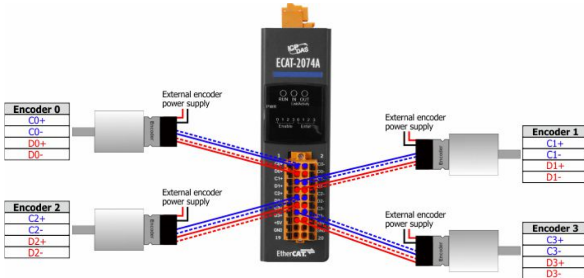
Figure 7: ECAT-2074A encoder connection
