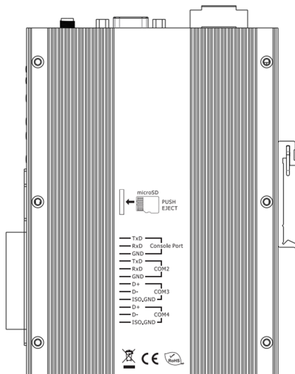
Figure 1-7 Appearance: BRK-2841M (2)
