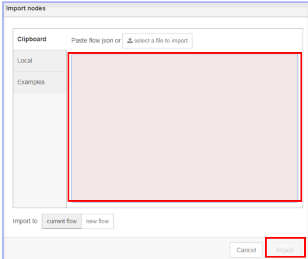
Figure 6-2 Import Page (2)
