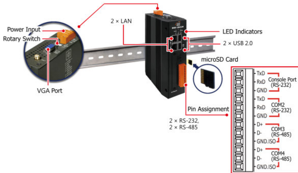
Figure 1-6 Appearance: BRK-2841M (1)
