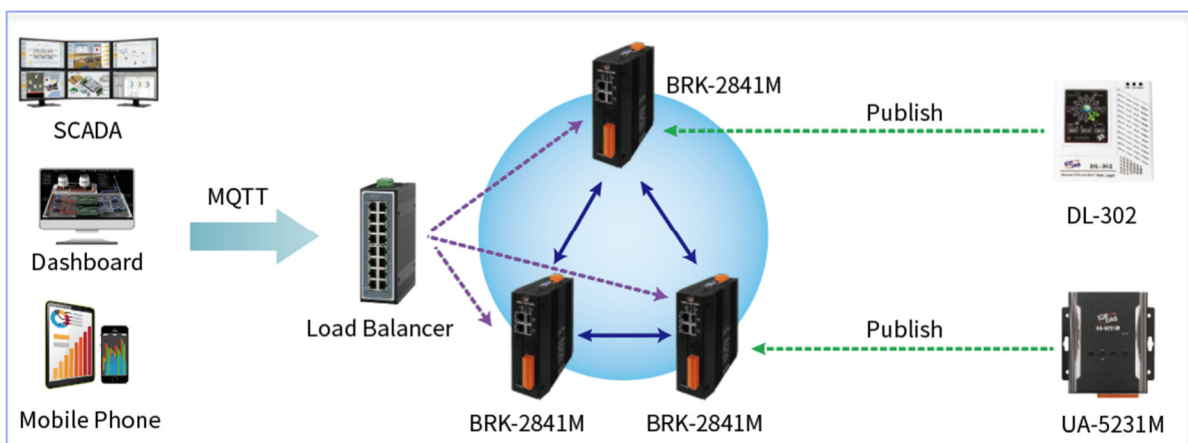
Figure 1-1 BRK-2841M Product Architecture
