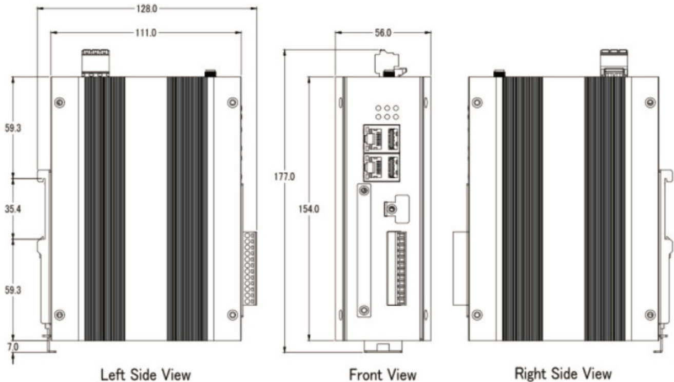
Figure 1-8 Dimensions: BRK-2841M
