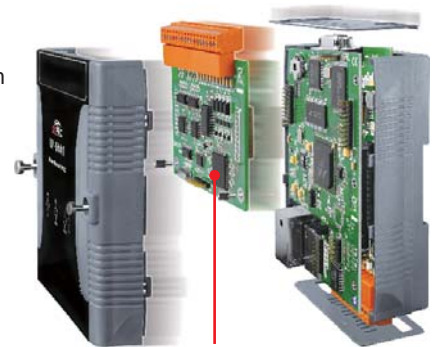
XV-Board or XW-Board
