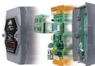
Plug an X-Board into a palm-size PAC
