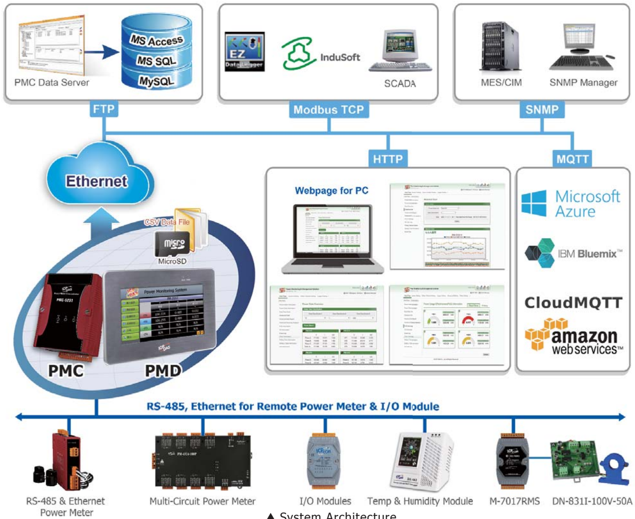
▲ System Architecture
