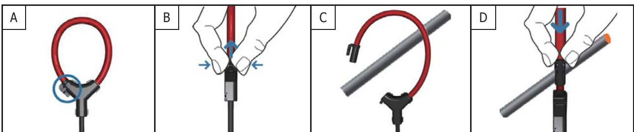
Rogowski coil Soft CT Installation
