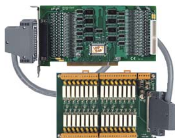
PISO-C64 with DB-32R: 32-ch relay (3A, Form A) board, 1m cable.
