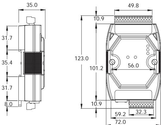
ET-7000/PET-7000 Series
