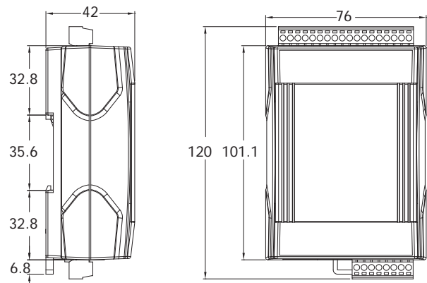
ET-7200/PET-7200 Series
