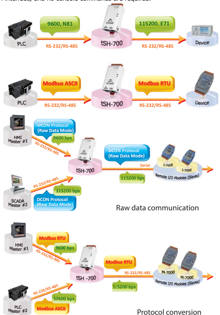
Protocol conversion
