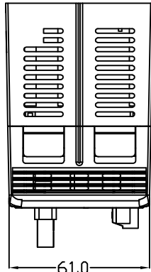
61.0 Top View
