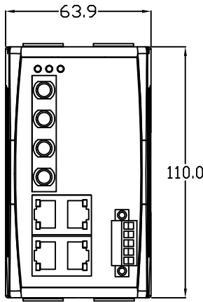
63.9 110.0 Front View
