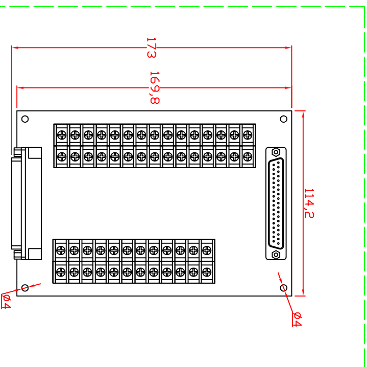
Front View (only PCB)
