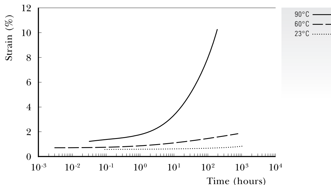
■ FIGURE 15 Creep performance of Cypoloy C1100 at 15 MPa
