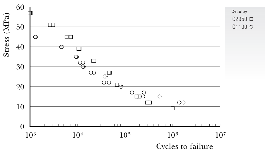
■ FIGURE 16 Fatigue performance of Cypoloy C1100 and C2950 at 23°C and 5 Hz
